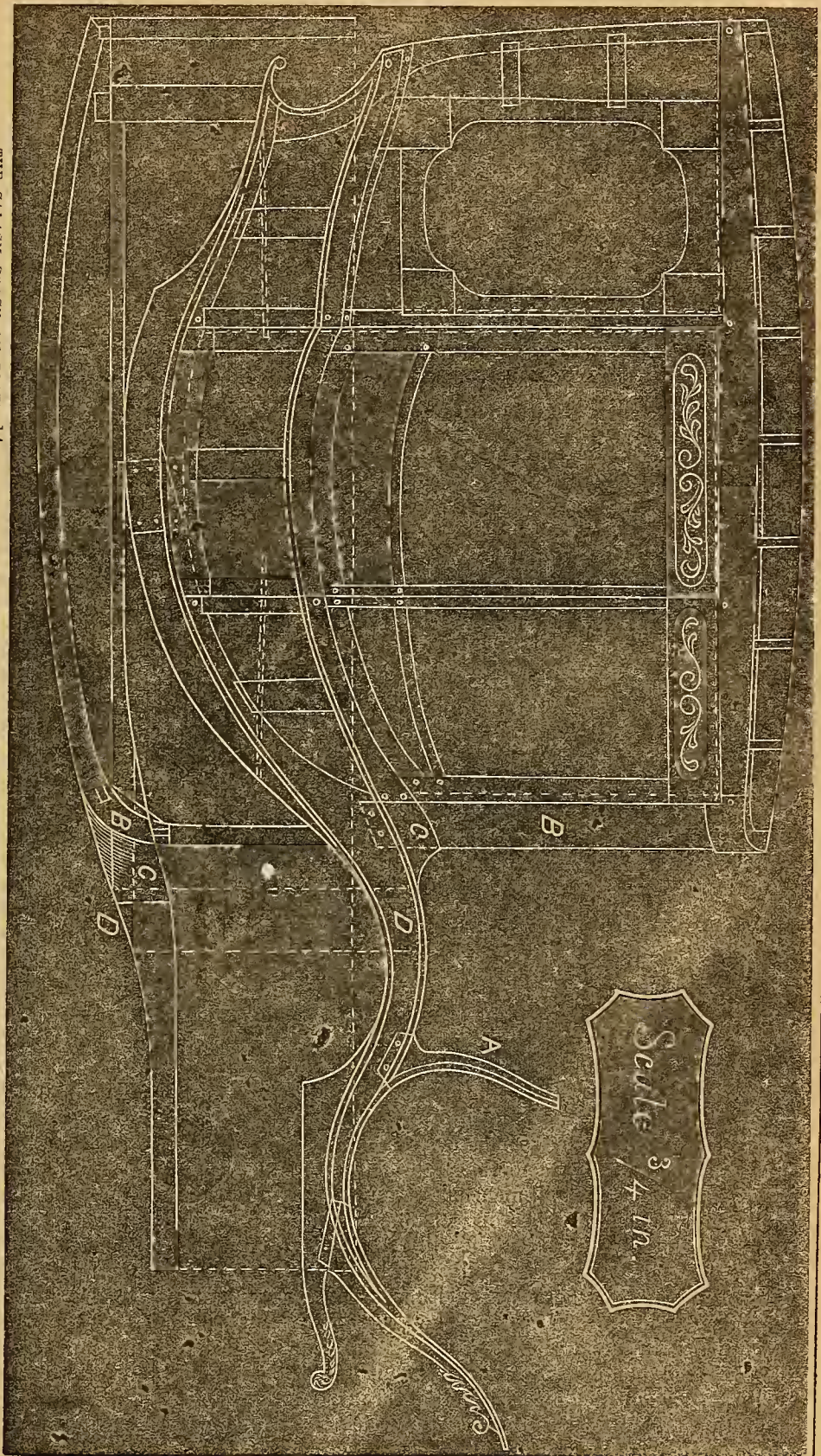
THE GALASH COACH ON PLATE 14, VOL. I, IN FRAME READY FOR PANELING—THE DIFFICULT POINTS OF CONSTRUCTION EXPLAINED.
